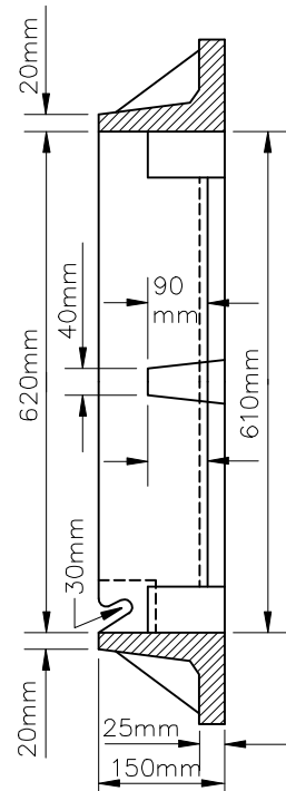
SECTION C-C
