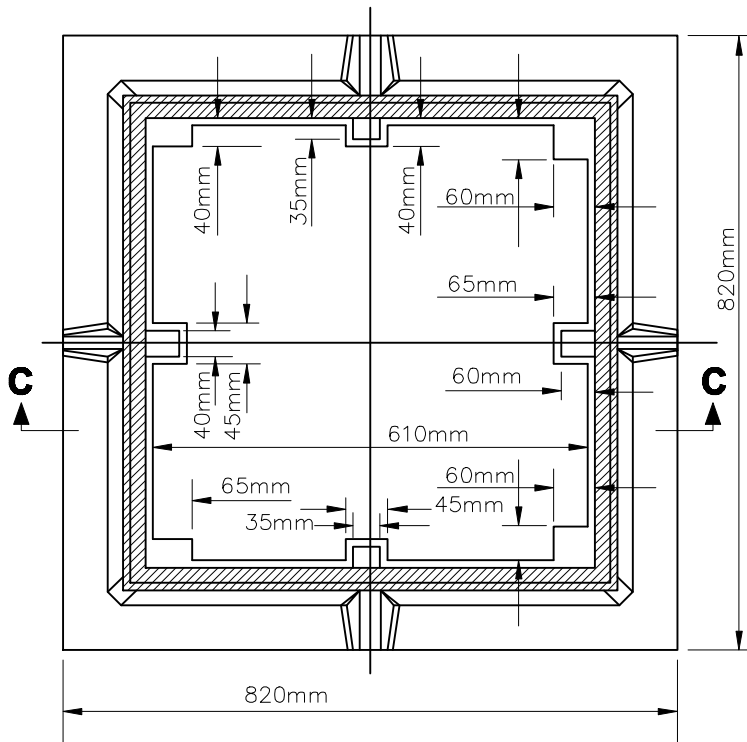
FRAME PLAN
