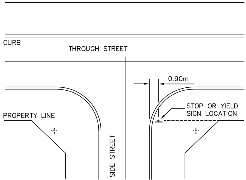
3-WAY INTERSECTION
