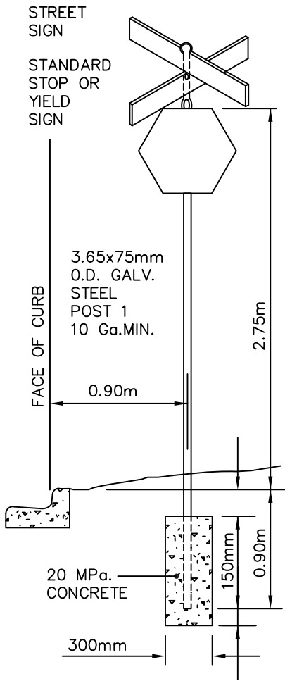
SIGN DETAIL
